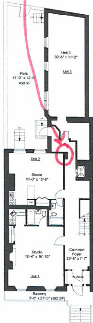
EXISTING FIRST FLOOR PLAN 1743 SF
