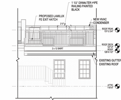
2 EAST PROPOSED Copy 1 1/4" = 1'-0"
