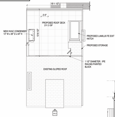
1 ROOF PLAN PROPOSED 1/4" = 1'-0"
