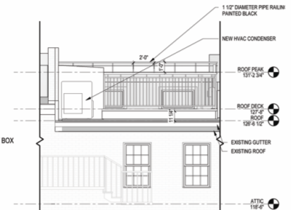
2 EAST PROPOSED Copy 1 1/4" = 1'-0"
