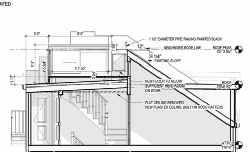
3 Section 1 Copy 1 1/4" = 1'-0"
