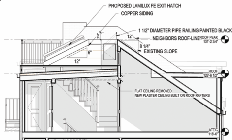
3 Section 1 Copy 1 1/4" = 1'-0"
