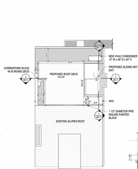
1 ROOF PLAN PROPOSED 1/4" = 1'-0"
